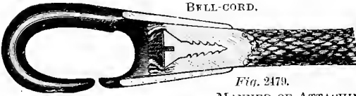
MANNER OF ATTACHING BELL-CORD TO COUPLING.
